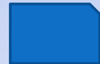
polygons
