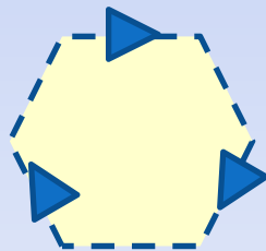
hexagonal
