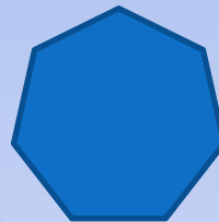
heptagon
