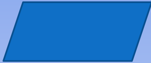
parallelogram
